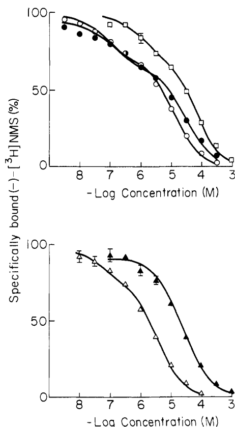
Figure 3. Competitive inhibition of (-)-[ 3 H]NMS binding in rat cerebral cortex by 8a (●), 6a (○), 6b (□), 7a (△), and 7b (▲). Values are means ± standard errors from three experiments, each performed in triplicate. The concentration of (-)-[ 3 H]NMS used was 0.3 nM. The theoretical curves are the least-squares fit to the data.
